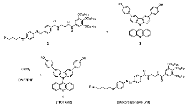
Figure 2. Synthesis and chemical structure of compound 1 : CsCO 3 (16 equiv), DMF/THF (4:3, v/v), 100 °C, 24 h, 65%.
