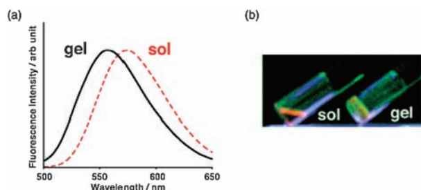
Figure 4. (a) Fluorescence spectra of 1 ( [1] = 4.0 mM, solvent: 1-decanol, \lambda_{\text{ex}} = 350 nm, optical path length: 1.0 mm, temperature: 25 °C.), (b) the image of 1 + 1-decanol sol and gel.
